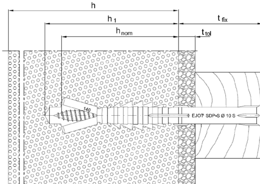
Picture 1: Intended use: screw head-type: countersunk (S)
